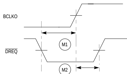
Figure 20-18. DMA Timing
