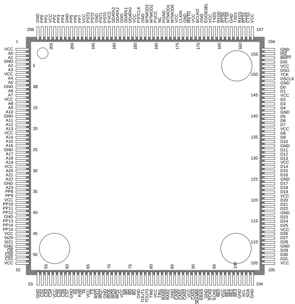
Figure 16-1. Mechanical Diagram
