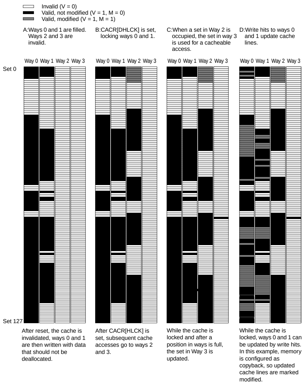
Figure 4-7. Cache Locking
