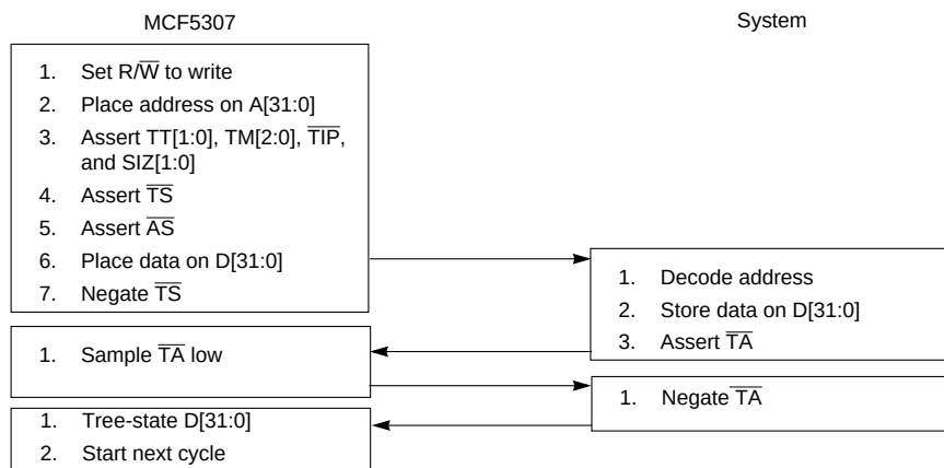
Figure 18-7. Write Cycle Flowchart
