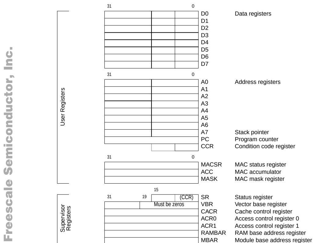
Figure 1-4. ColdFire MCF5307 Programming Model
