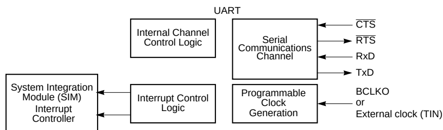
Figure 14-1. Simplified Block Diagram
