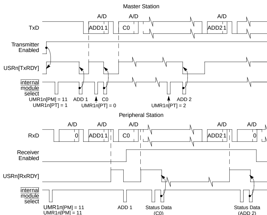
Figure 14-26. Multidrop Mode Timing Diagram
