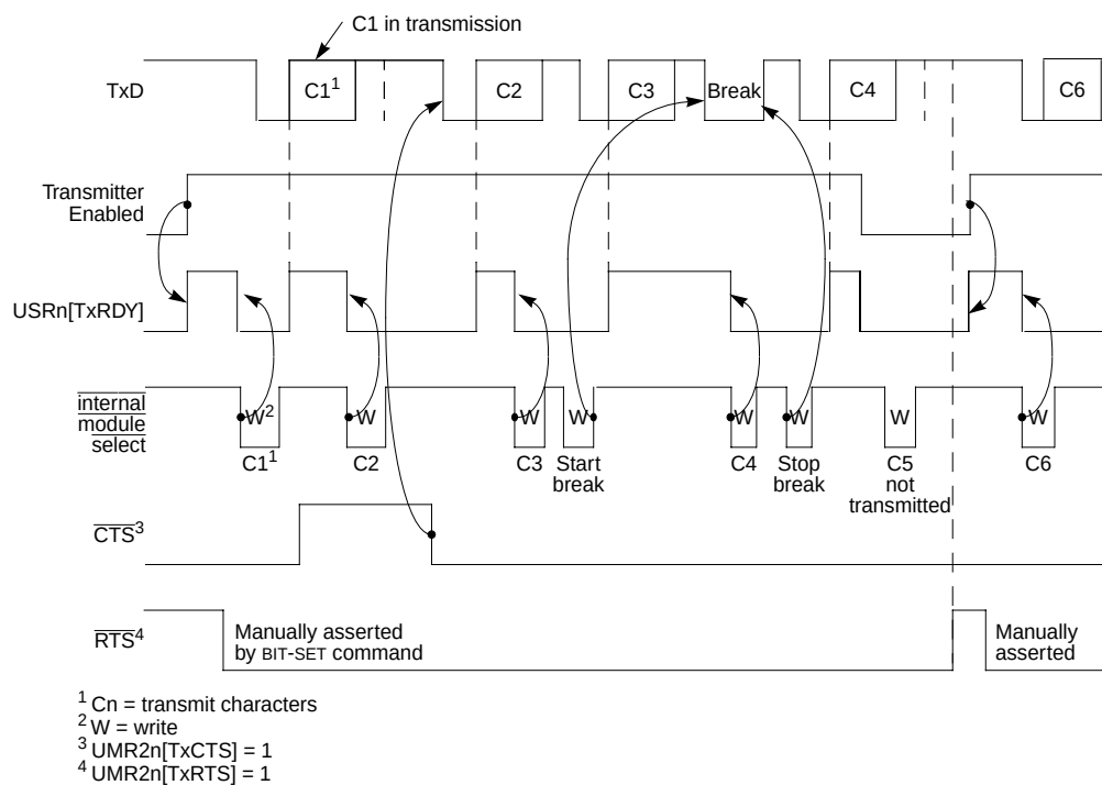
Figure 14-21. Transmitter Timing Diagram
