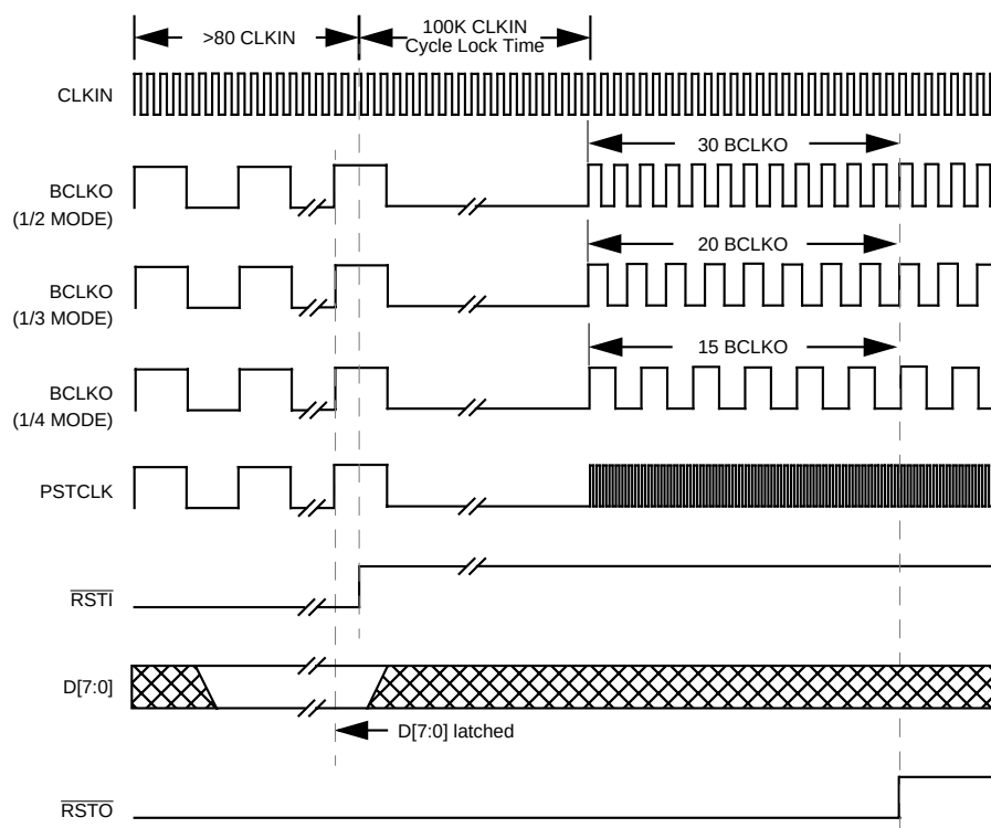
Figure 18-34. Software Watchdog Reset Timing
