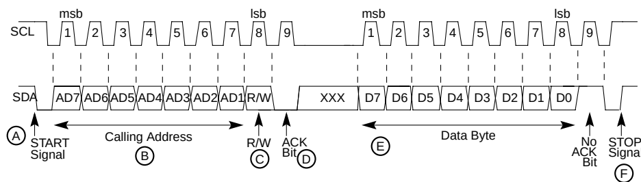
Figure 8-2. I 2 C Standard Communication Protocol
