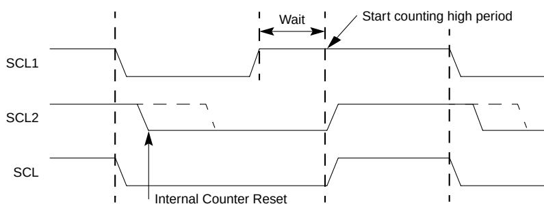
Figure 8-4. Synchronized Clock SCL
