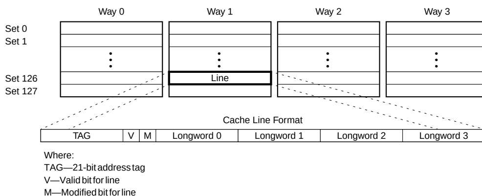
Figure 4-3. Cache Organization and Line Format
