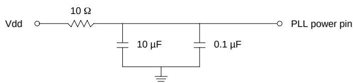
Figure 7-5. PLL Power Supply Filter Circuit
