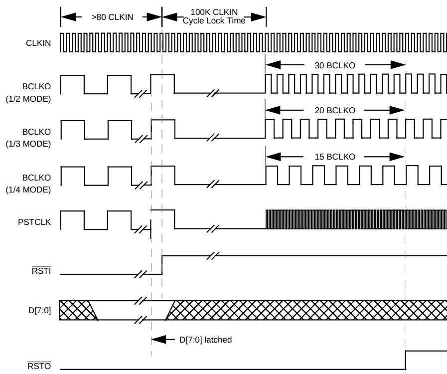
Figure 7-4. Reset and Initialization Timing
