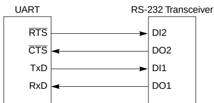
Figure 14-18. UART/RS-232 Interface
