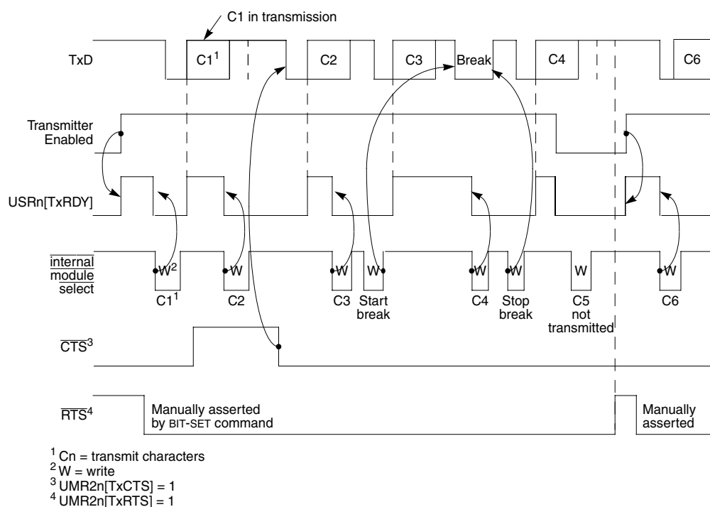
Figure 14-30. Transmitter Timing Diagram
