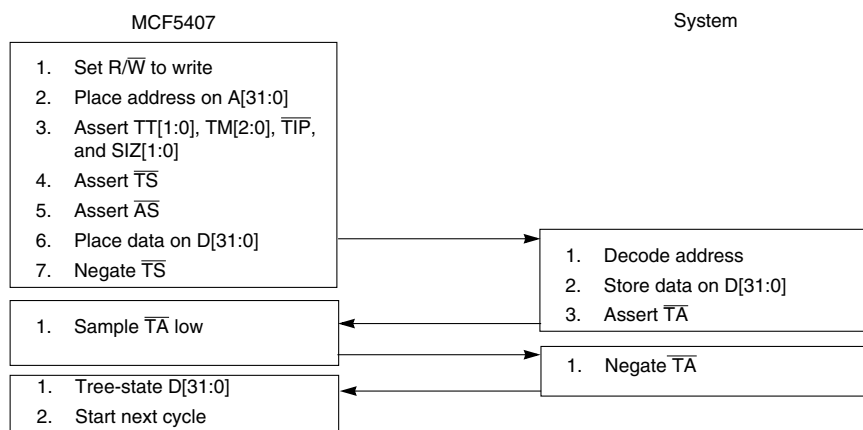
Figure 18-7. Write Cycle Flowchart
