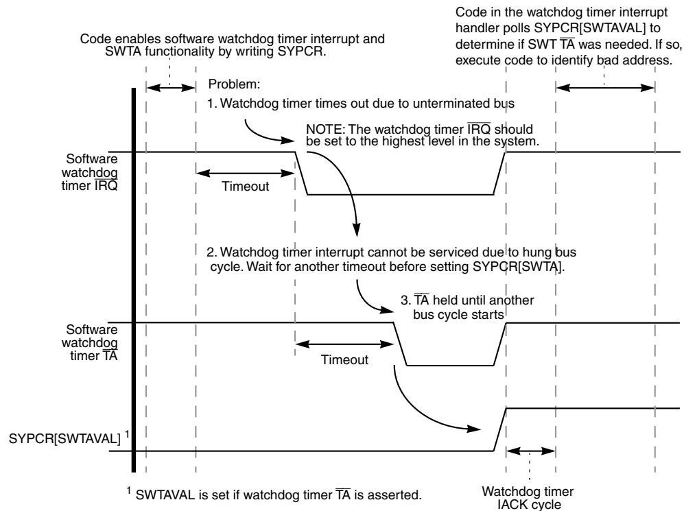
Figure 6-4. MCF5407 Embedded System Recovery from Untermiated Access
