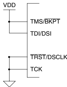
Note: MTMOD0 high allows JTAG mode. Figure 19-4. Disabling JTAG in JTAG Mode
