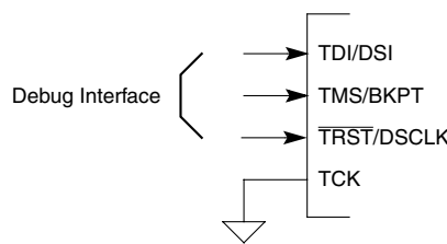
Note: MTMOD0 low prohibits JTAG. Figure 19-5. Disabling JTAG in Debug Mode
