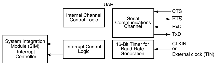
Figure A-2. Simplified Block Diagram
