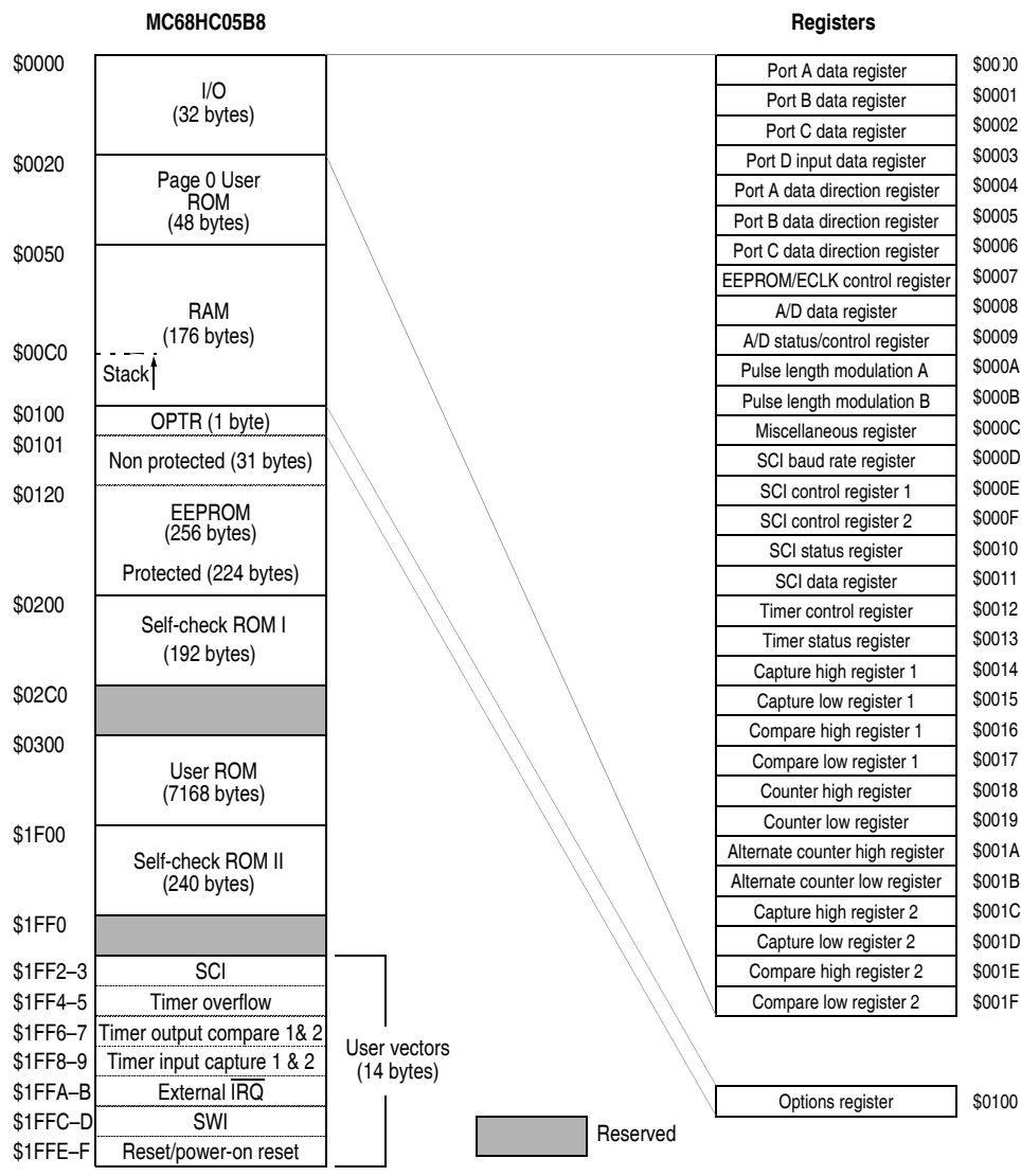
Figure B-2 Memory map of the MC68HC05B8
