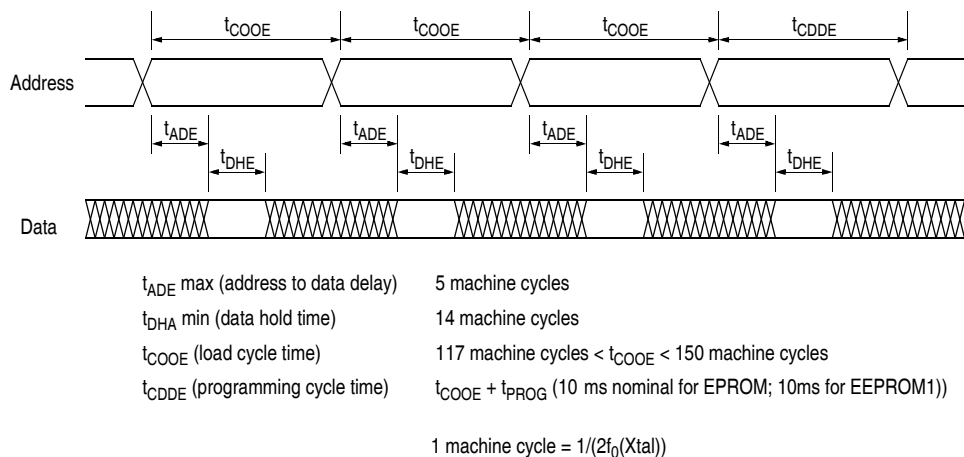
Figure F-6 Parallel EPROM loader timing diagram
