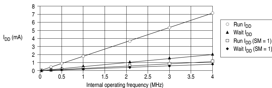
Figure 11-6 I_{DD} vs mode vs internal operating frequency, V_{DD} = 5.5V
