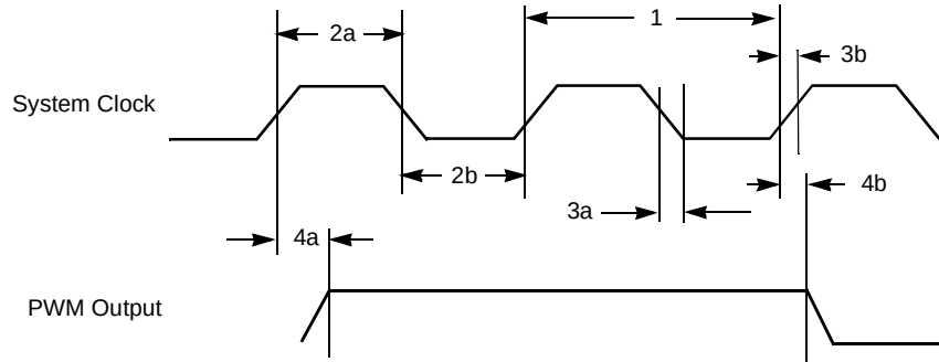
Figure 70. PWM Timing
