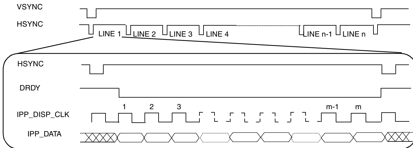
Figure 53. Interface Timing Diagram for TFT (Active Matrix) Panels
