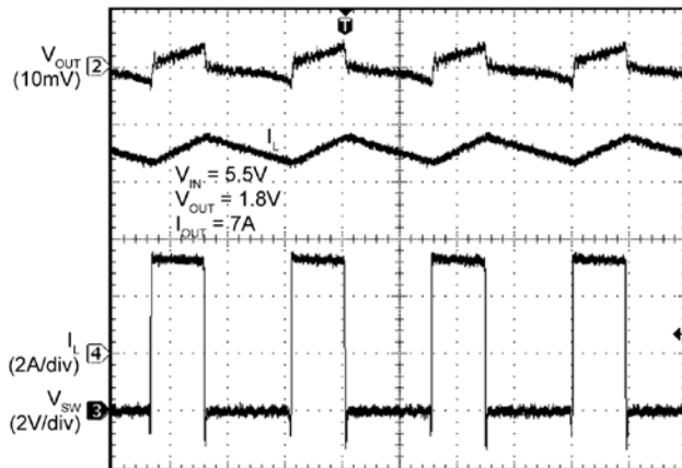
Switching Waveforms
