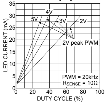
LED Current vs. Duty Cycle
