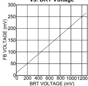
FB Voltage vs. BRT Voltage
