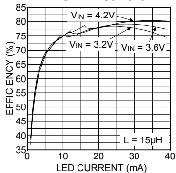
Efficiency for 10 LEDs vs. LED Current
