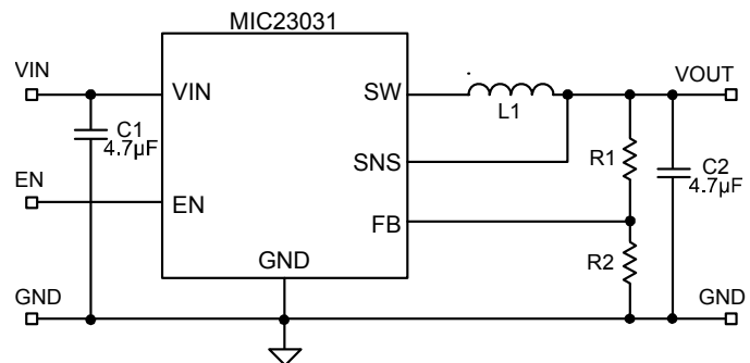
Figure 1. MIC23031-AYMT Schematic
