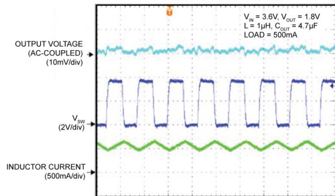
Switching Waveform Continuous Mode – 500mA
