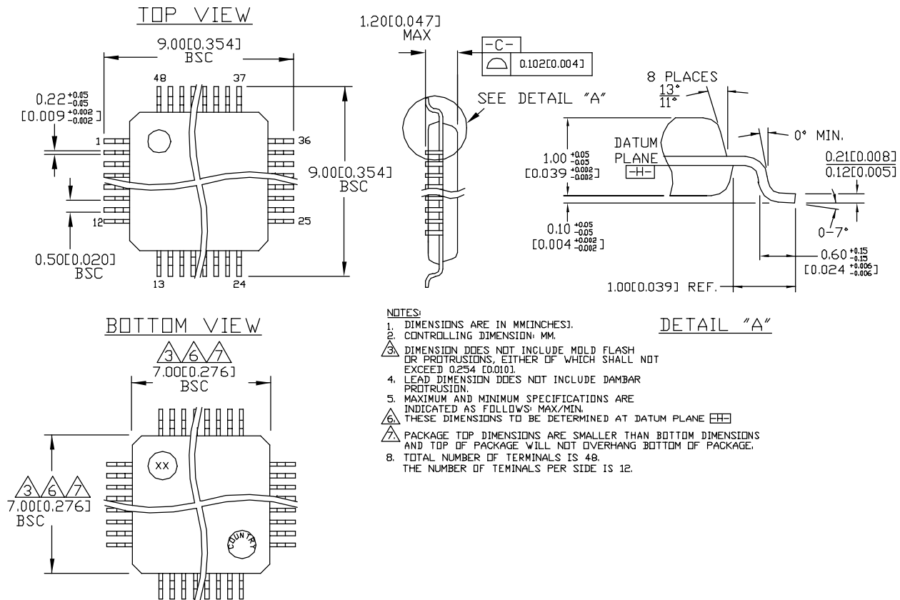
48-Pin TQFP
