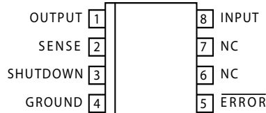
MIC29201-3.3BM (SOIC-8)
