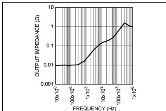
FIGURE 2-81: MIC2975x Output Impedance vs. Frequency.
