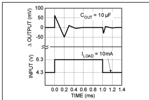
FIGURE 2-79: MIC2975x Line Transient.
