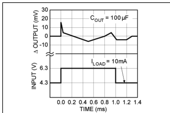
FIGURE 2-80: MIC2975x Line Transient.
