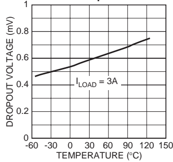
MIC2931x Dropout Voltage vs. Temperature
