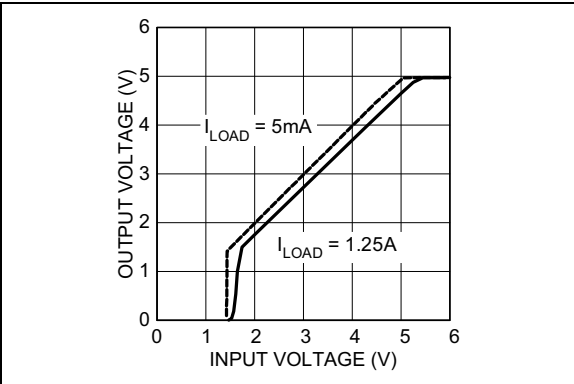
FIGURE 2-3: Dropout Characteristics.
