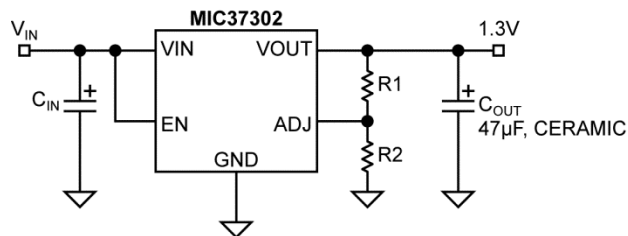
Adjustable Regulator
