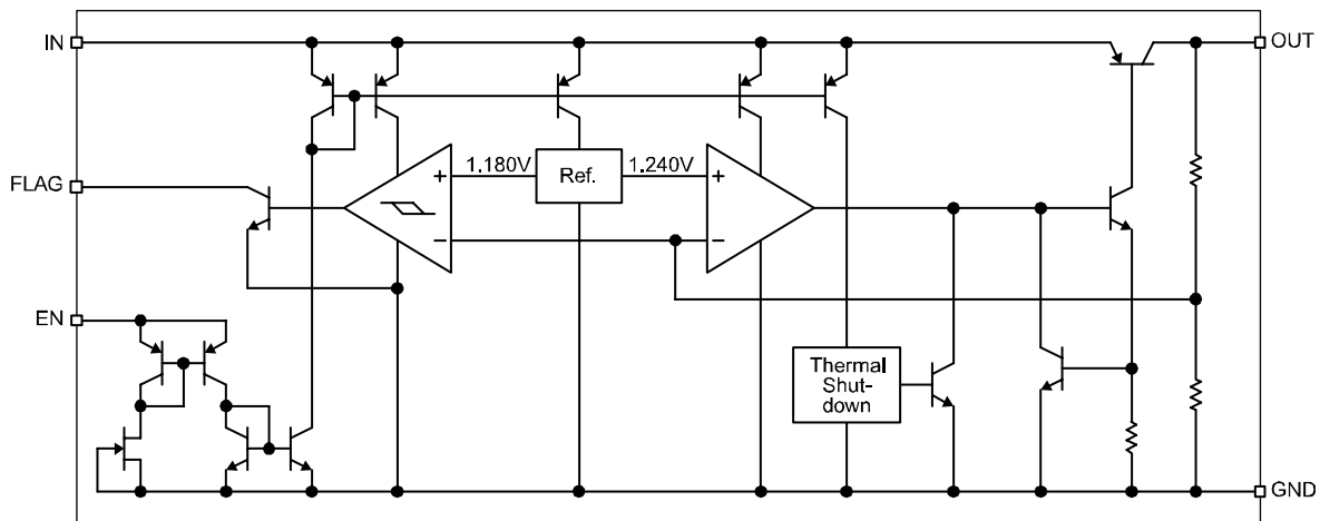
MIC3775 Fixed Regulator with Flag and Enable Block Diagram
