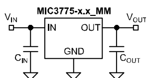
Figure 1. Capacitor Requirements
