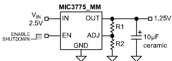
1.25V/750mA Adjustable Regulator
