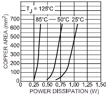
Figure 5. Copper Area vs. Power-MSOP Power Dissipation (T A )
