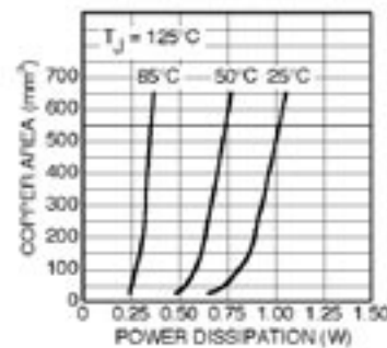
Figure 5. Copper Area vs. Power-MSOP Power Dissipation ( T_J )
