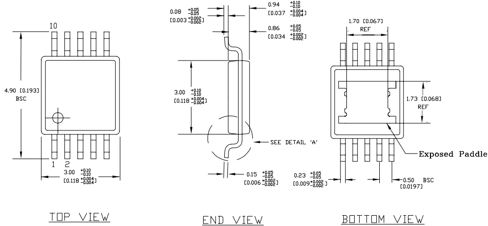
END VIEW
