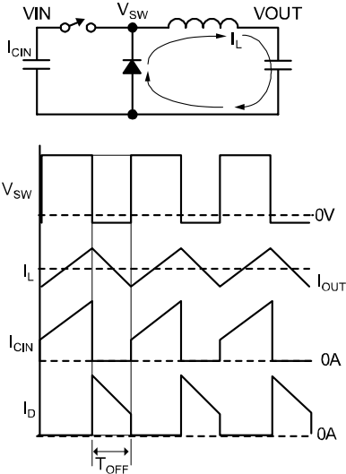
Figure 4. Off-Time
