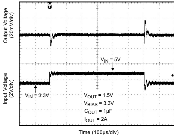
Line Transient ( V_{IN} )
