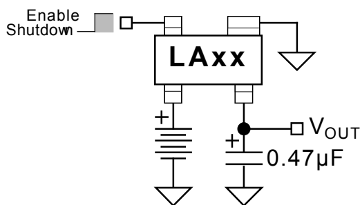
SOT-143 Version
