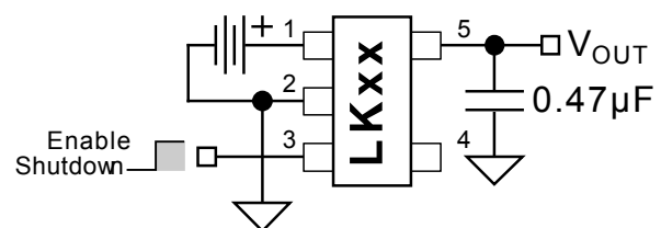
SOT-23-5 Version
