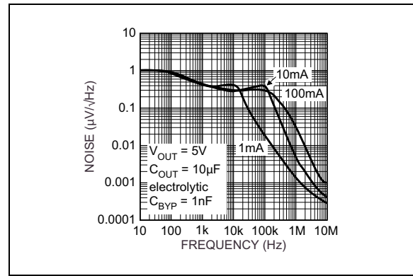
FIGURE 2-17: Noise Performance.
