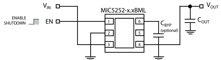
Ultra-Low-Noise Regulator Application
