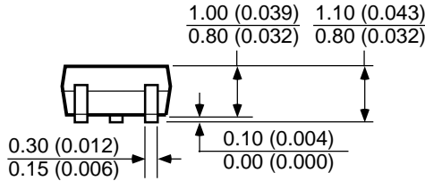
5-Pin SC-70-5 (C5)
