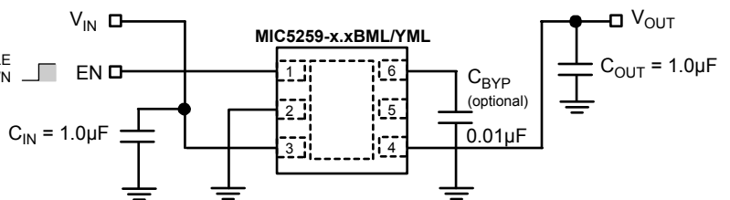
Ultra-Low Noise Regulator Application
