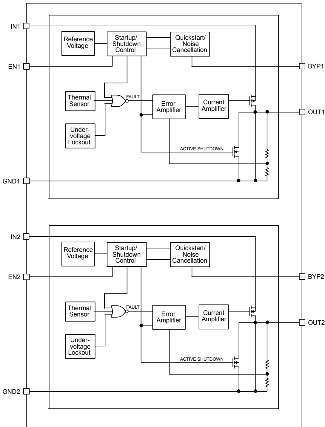
MIC5264 Diagram
