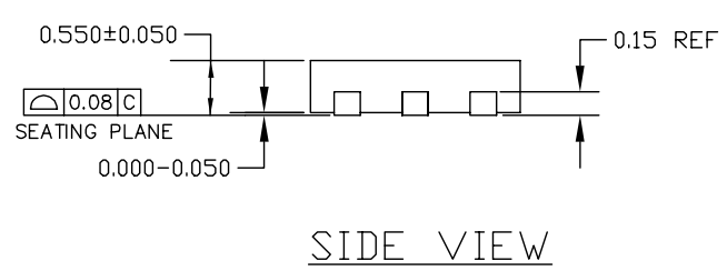
6-Pin 2x2 Thin MLF ® (MT)
