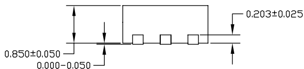
SIDE VIEW
