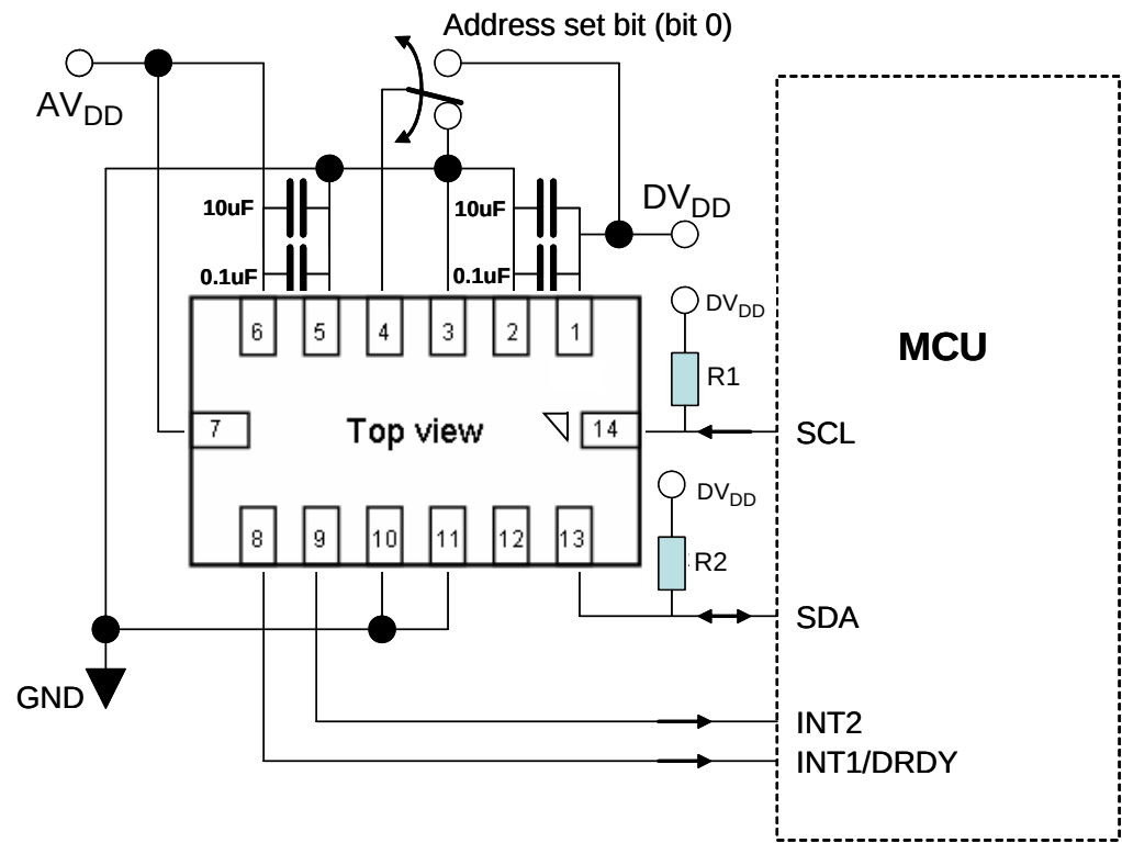
Figure 15. I 2 C Connection to MCU
