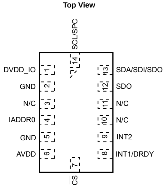
Figure 14. Pinout Description
