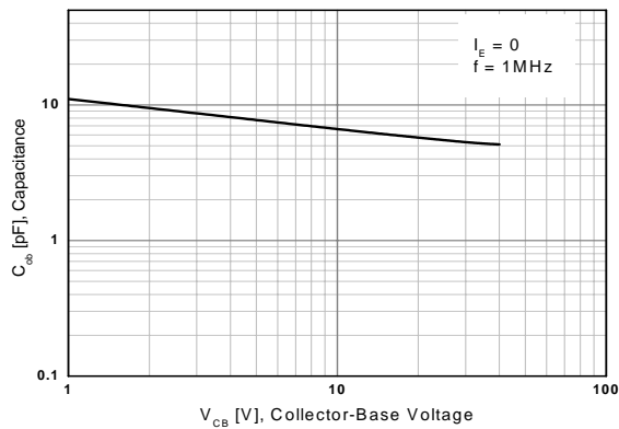
Figure 5. Output Capacitance
