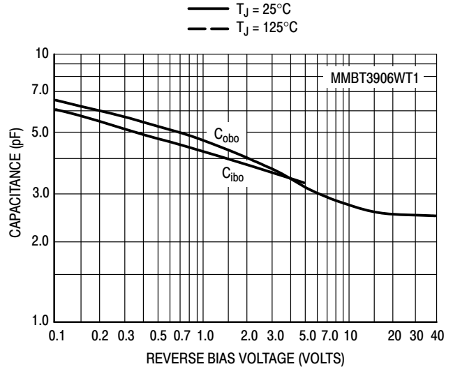
Figure 38. Capacitance
