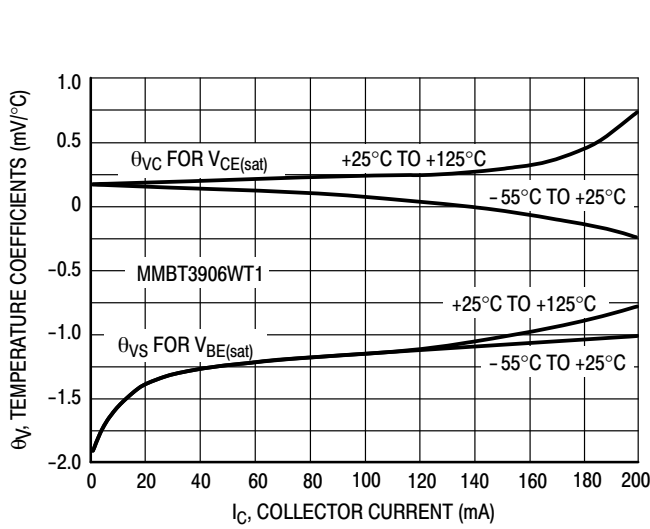
Figure 37. Temperature Coefficients
