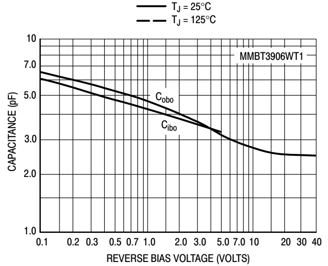
Figure 38. Capacitance
