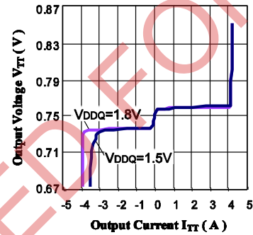
DDR3 Regulation
