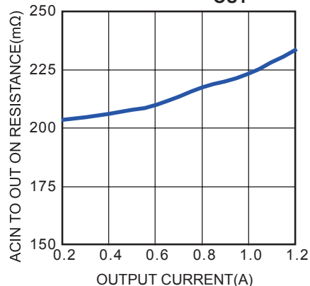
ACIN to OUT On Resistance vs. I_{\text{OUT}}
