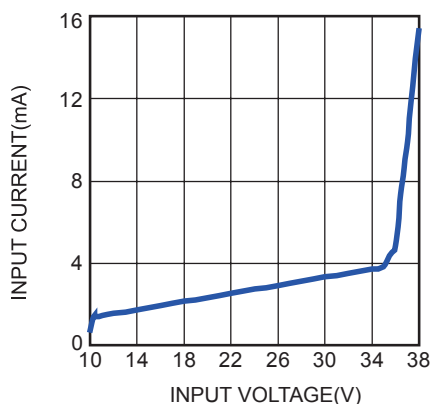
Breakdown Voltage
