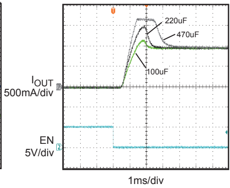
Inrush Current with Different Load Capacitance I_{OUT}=1A
