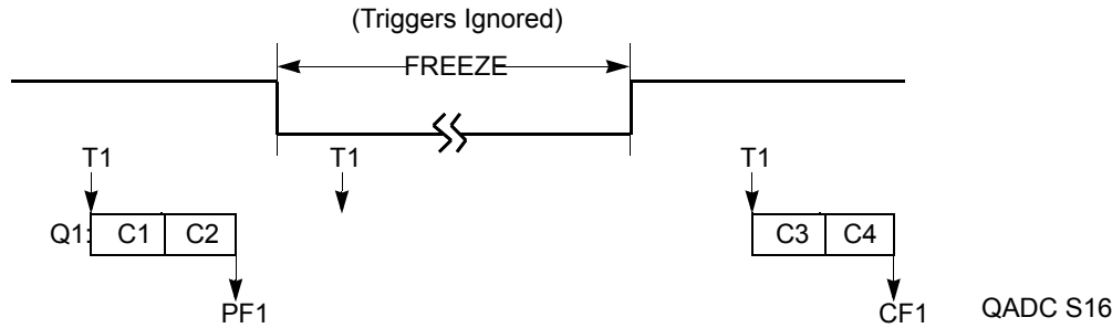
Figure 13-42. CCW Freeze Situation 16
