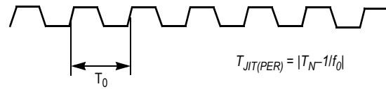
Figure 20. I/O Jitter
