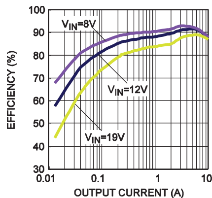
Figure 18 — Efficiency Curve
