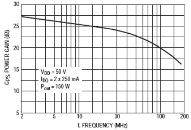
Figure 8. Power Gain versus Frequency
