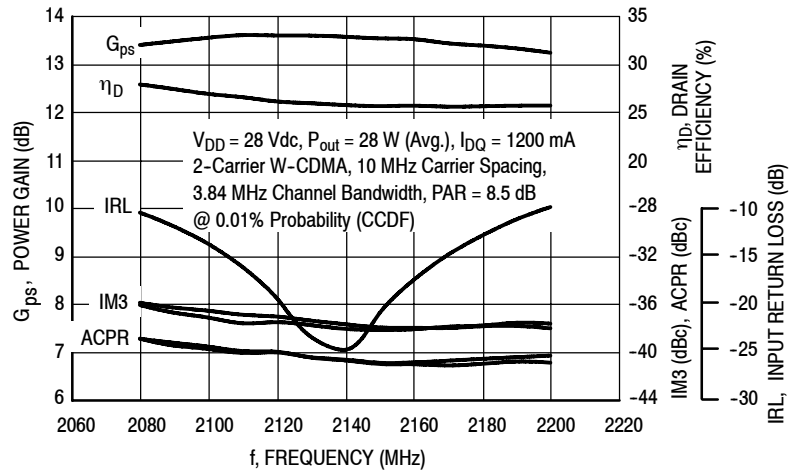
Figure 3. 2-Carrier W-CDMA Broadband Performance @ P out = 28 Watts Avg.
