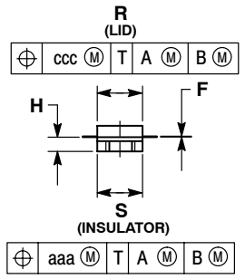
CASE 360C-05 ISSUE E NI-360S MRF9060LSR1
