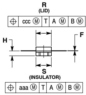
CASE 360B-05 ISSUE G NI-360 MRF9060LR1
