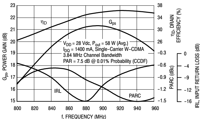
Figure 3. Single-Carrier W-CDMA Broadband Performance @ P out = 58 Watts Avg.
