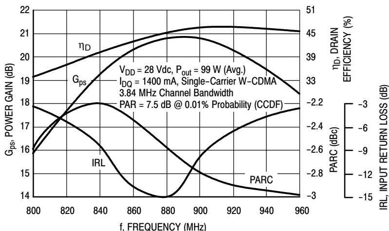
Figure 4. Single-Carrier W-CDMA Broadband Performance @ P out = 99 Watts Avg.
