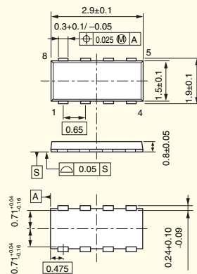
Package dimensions
