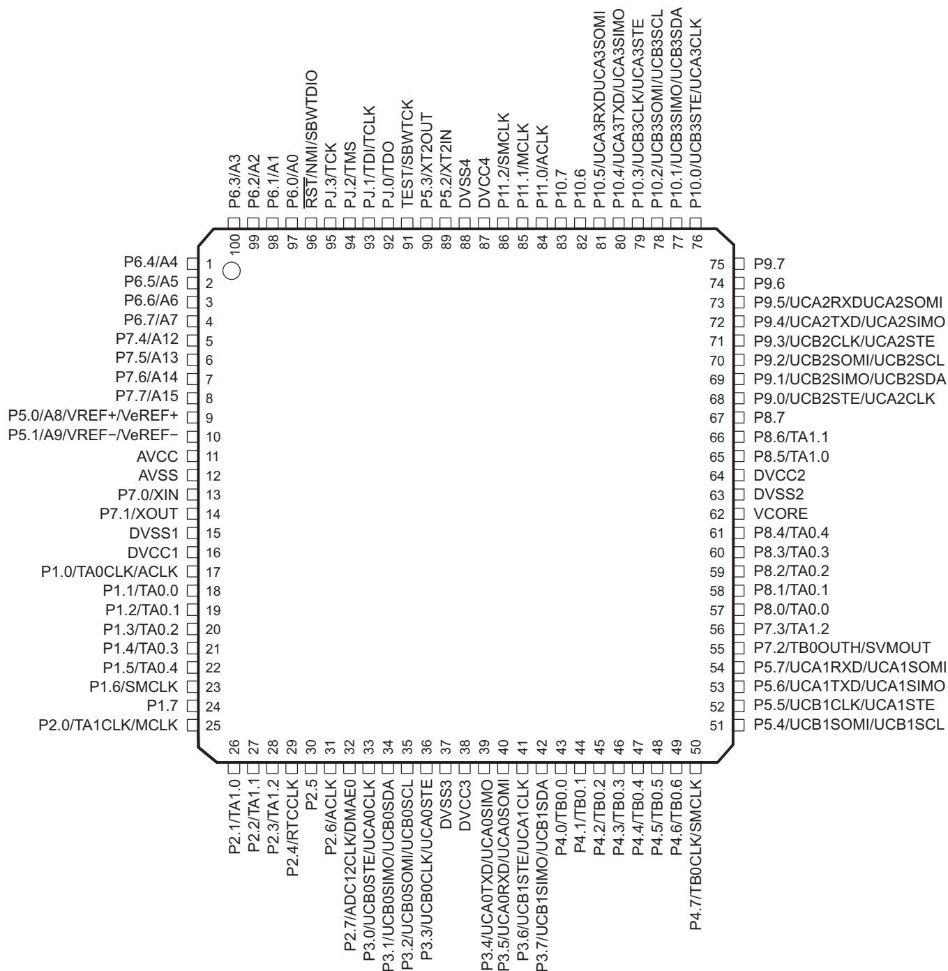
Figure 4-1. 100-Pin PZ Package (Top View)
