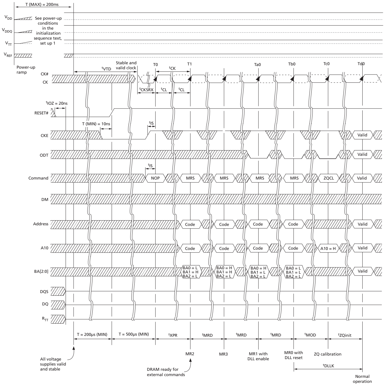
Figure 48: Initialization Sequence
