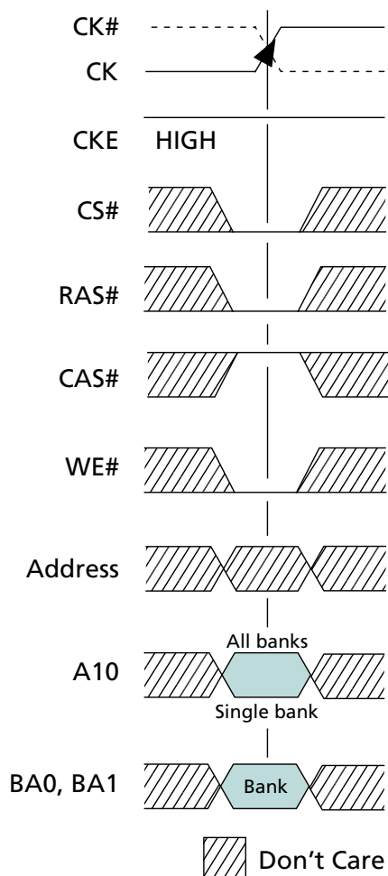
Figure 21: PRECHARGE Command
