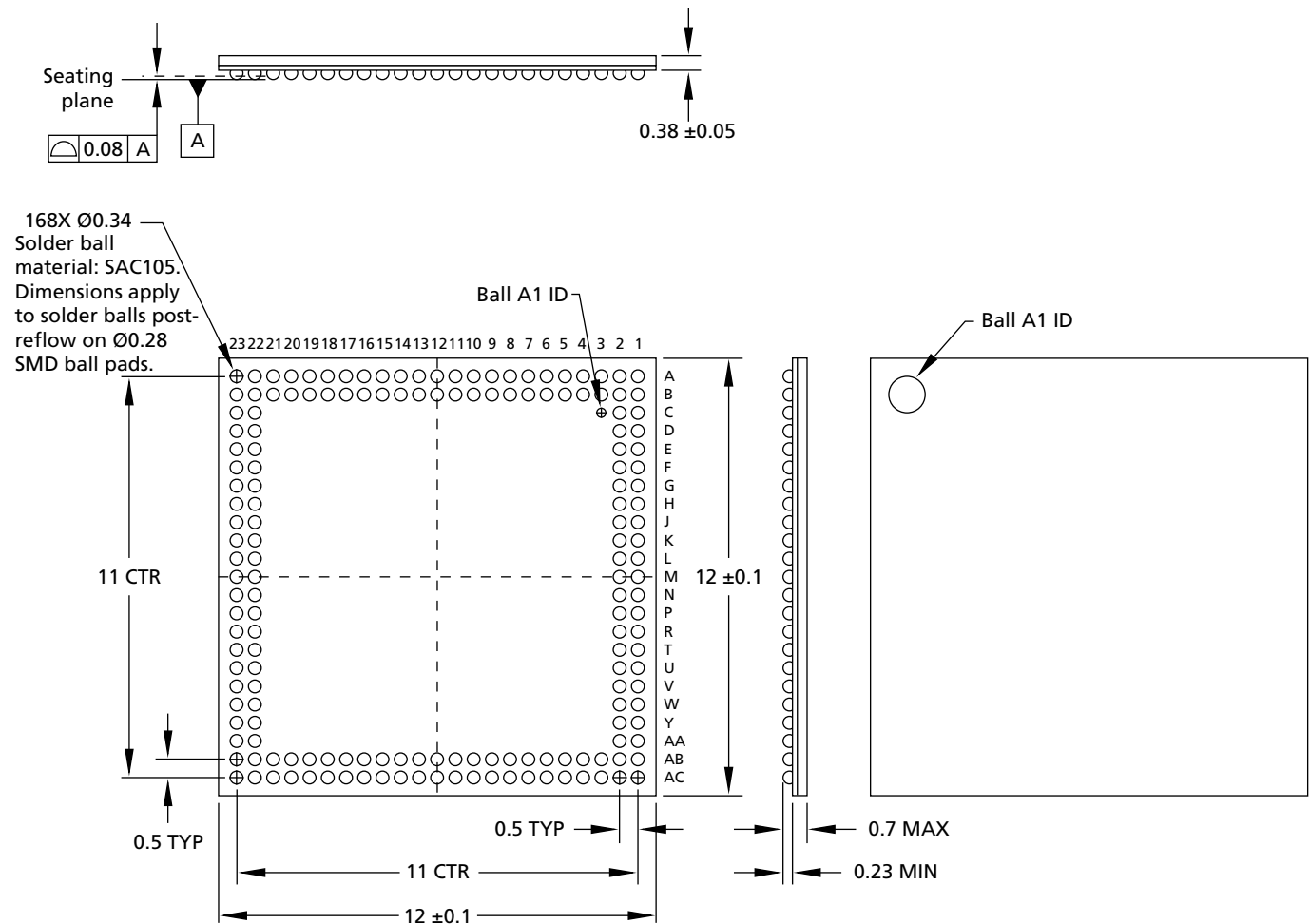
Figure 15: 168-Ball WFBGA (12mm x 12mm), Package Code: MA
